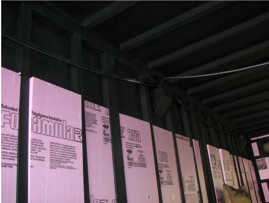
Mid to High Frequency Absorption - 2” Foam Board
